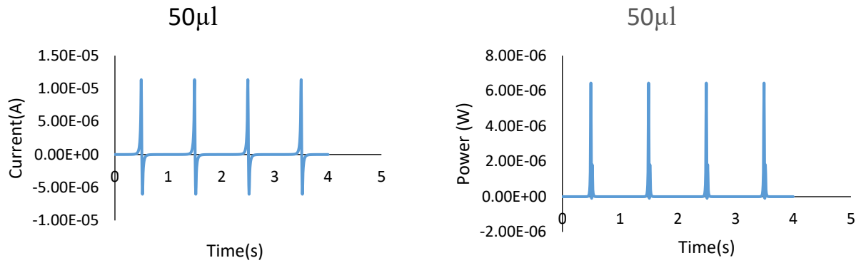
Fig. 11. Power output and generated current at different droplet volumes; bias ls voltages=5v, f=1\text{Hz} , d_1=d_3=1\mu\text{m} , k_1=k_3=2.8
