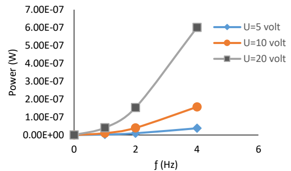
Fig. 9. Power output at different frequencies and bias voltages; R=50 \text{ k}\Omega , V=5 \text{ }\mu\text{L} , d_1=d_3=1 \text{ }\mu\text{m} , k_1=k_3=2.8
